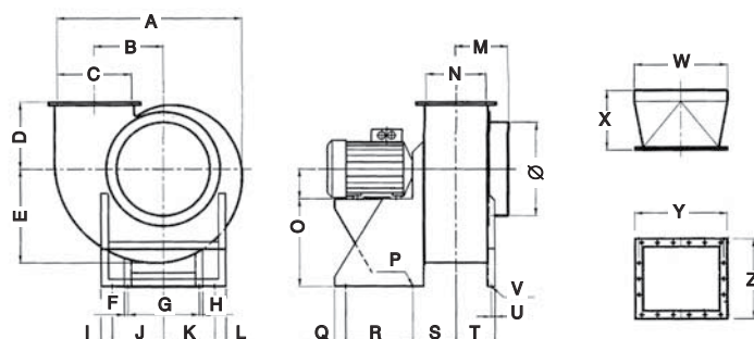
Dimenzije / Dimensions
